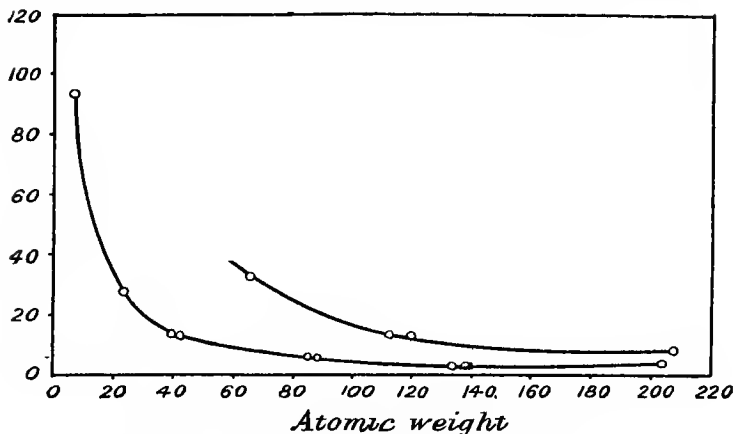
FIG. 101.—Atomic diffusivities of metals in mercury.
